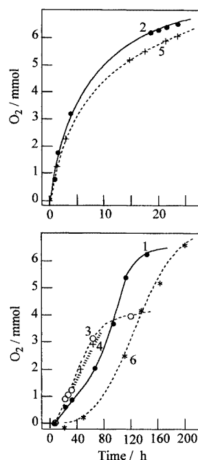
Figure 4. Consumption of O 2 in reaction of 2-methylcyclohexanone (7.6 mmol) in MeCN (total volume of reaction solution 6 mL), catalysed by [ n Bu 4 N]VO 3 (0.076 mmol) at 63 °C without additives (curve 1) and with PTSA (0.155 mmol) (2), CH 3 COOH (0.32 mmol) (3), PCA (0.306 mmol) (4), PTSA (0.155 mmol) + PCA (0.306 mmol) (5), and pyridine (0.755 mmol) (6)
