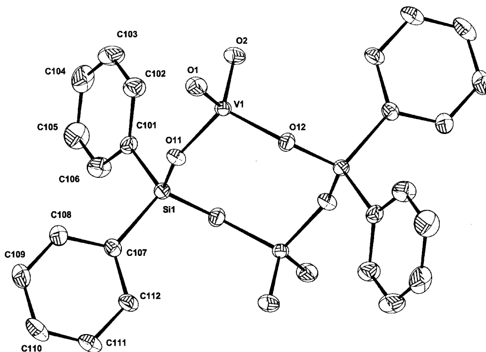
Figure 3. CAMERON representation [61] (ellipsoids at 30% probability level) of [\{\text{Ph}_2\text{SiO}_2\text{VO}_2\}_2]^{2-} , showing the atom-labelling scheme (H atoms omitted for clarity)
