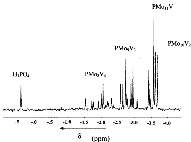
Figure 1. ^{31}\text{P} NMR spectrum of " \text{H}_6[\text{PMo}_9\text{V}_3\text{O}_{40}] " ( 1 \text{ mol} \cdot \text{dm}^{-3} ; pH 0.8) prepared by treatment of \text{MoO}_3 \cdot x\text{H}_2\text{O} , \text{V}_2\text{O}_5 and \text{H}_3\text{PO}_4 with \text{H}_2\text{O}_2 at room temperature (the identification is supported by solutions and solids prepared with 2 \leq n \leq 10 – see ref. [5,7,47] )
